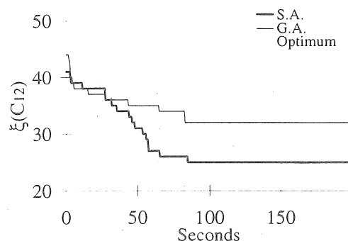
Figure 2: Experimental comparison with a genetic algorithm. For each second, we plot the best solution obtained so far by the simulated annealing algorithm (S.A.) and by the genetic algorithm (G.A.)
